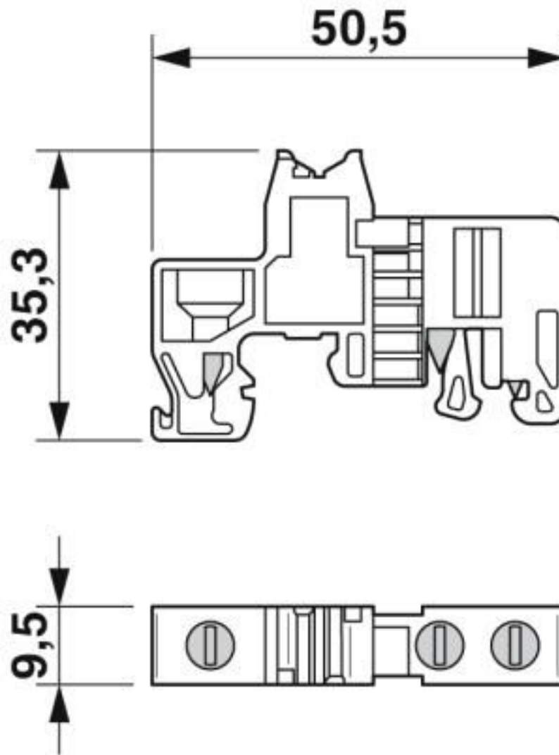
Dimensional drawing
